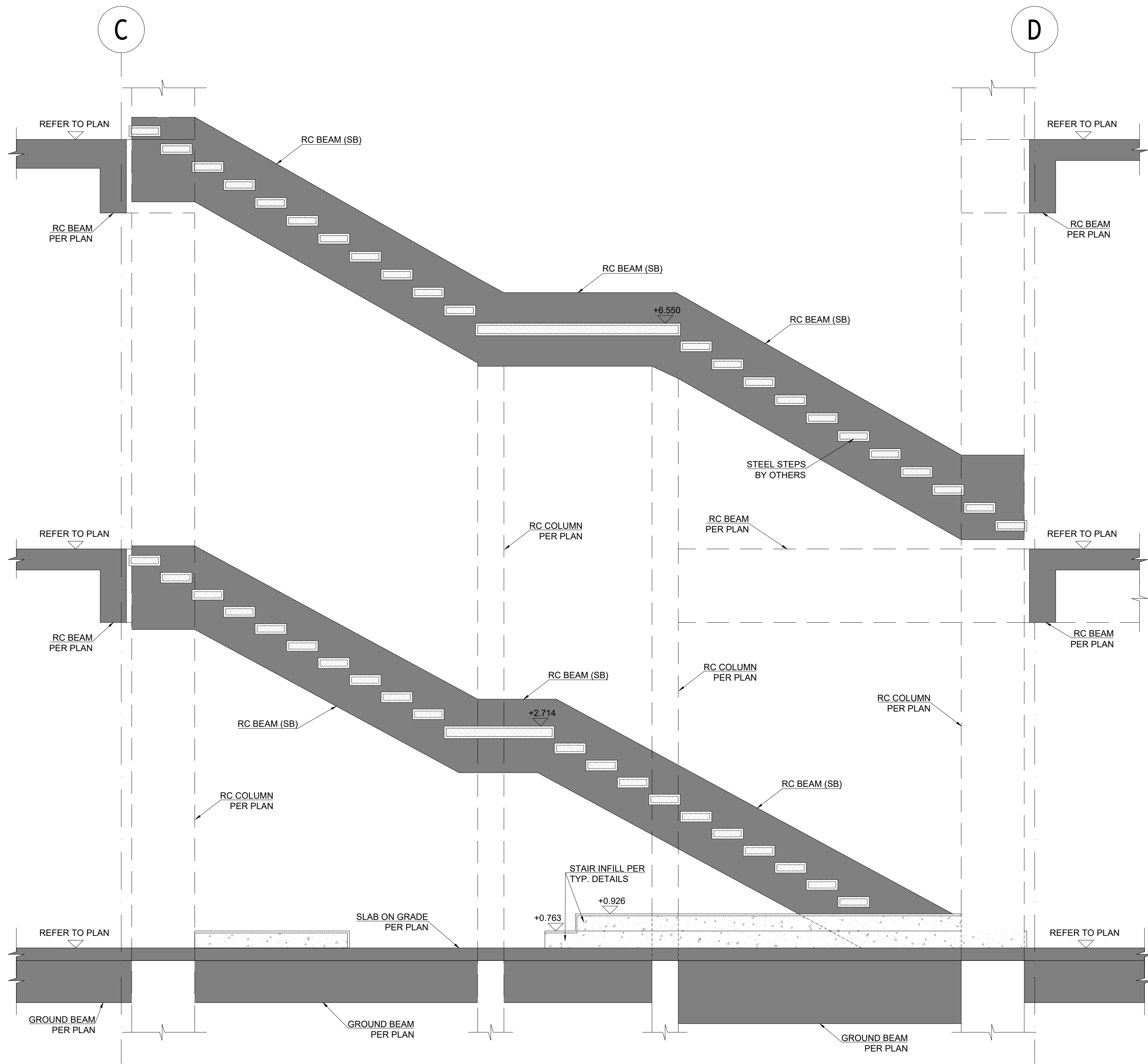
STAIRCASE SECTION
